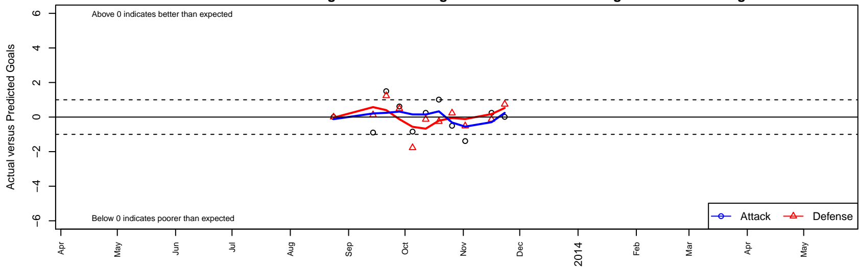
Flyers – Unk B00 Dots are actual minus expected GF (blue circles) and GA (red triangles). Blue line is smoothed change in attack strength. Red is smoothed change in defense strength.
